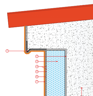
CORTE VERTICAL
