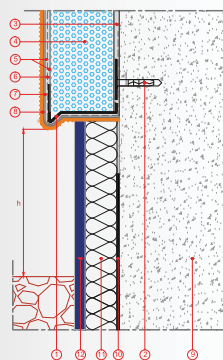
CORTE VERTICAL
