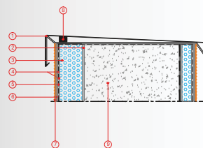
CORTE VERTICAL
