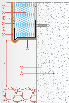
CORTE VERTICAL
