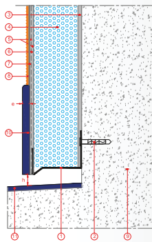
CORTE VERTICAL
